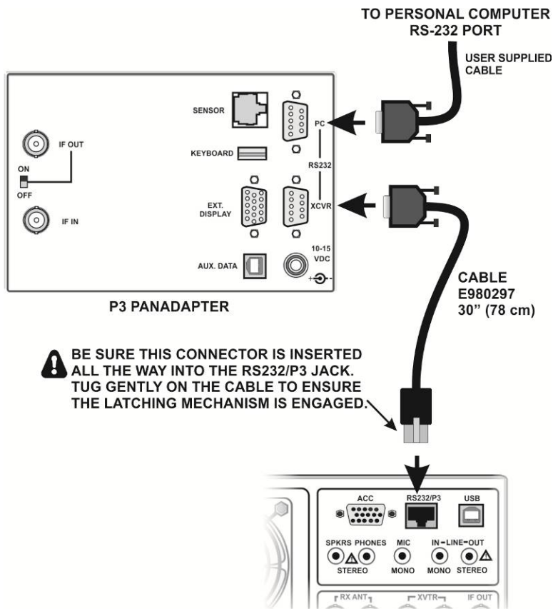
Figure 13. P3 Cabling for RS232 Computer Interface.
