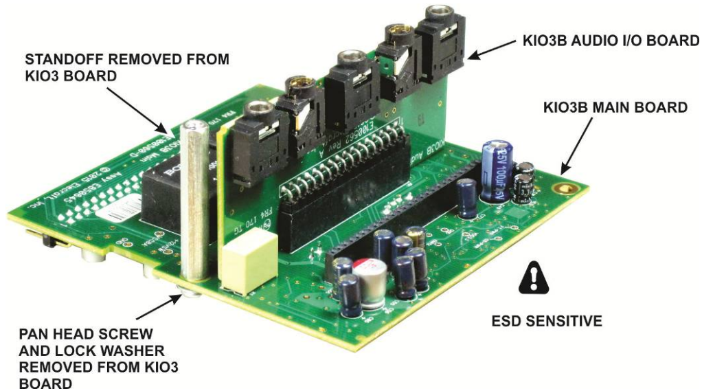
Figure 6. Mounting the Standoff and Audio I/O Board on the KIO3B Main Board.
