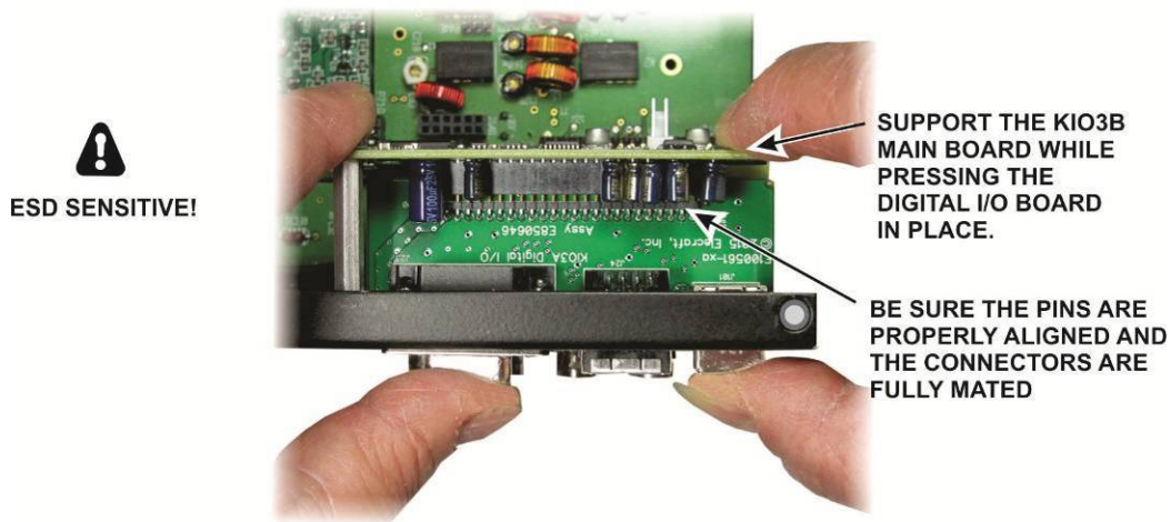
Figure 7. Installing the KIO3 Digital I/O Board.
