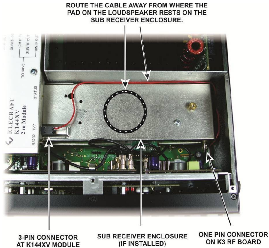
Figure 11. K144XV Power Cable Routing.
