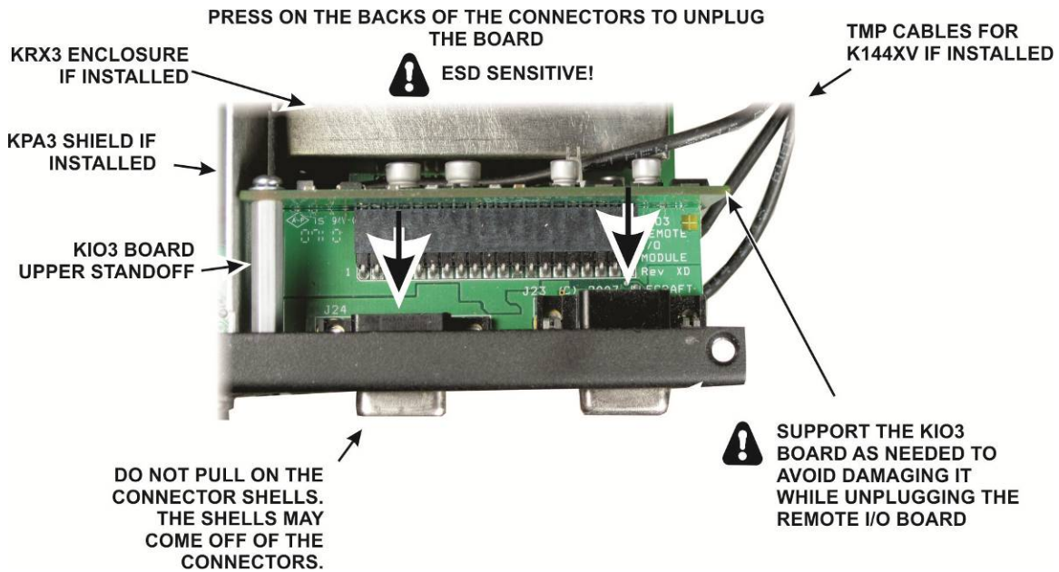
Figure 4. Removing the Remote I/O Board.
