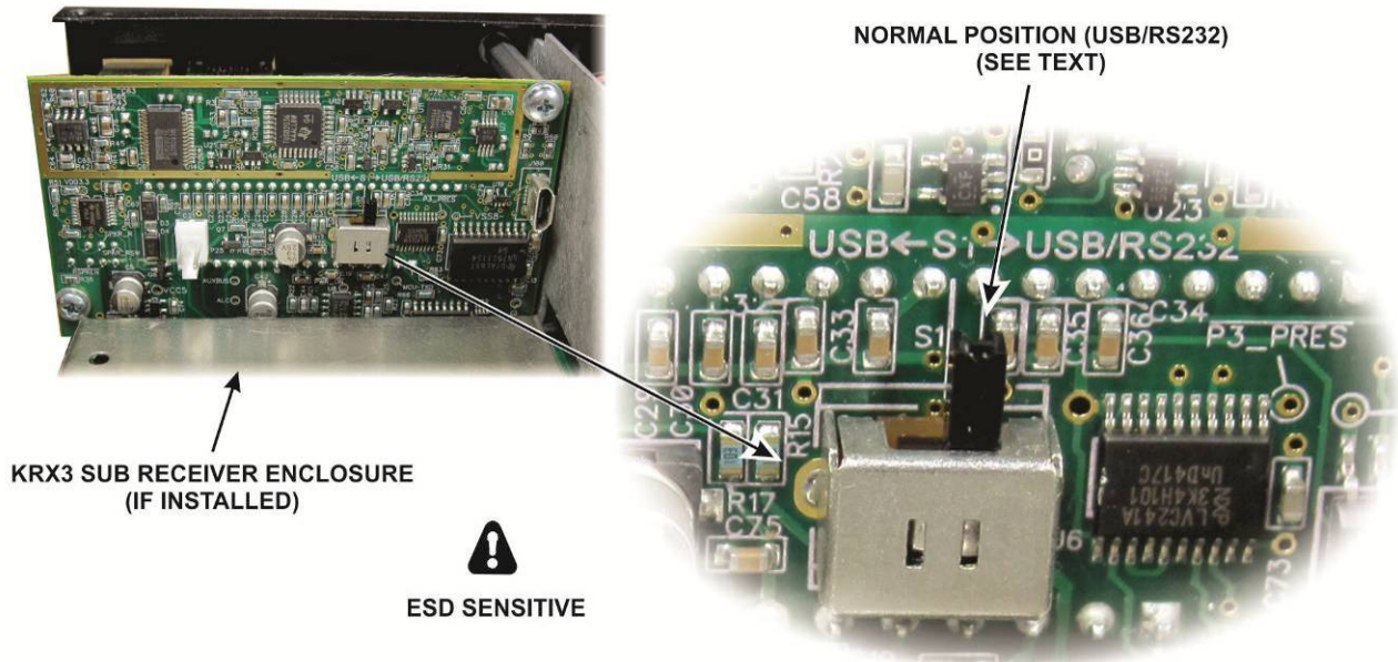
Figure 9. KIO3B USB/RS232 Switch.
