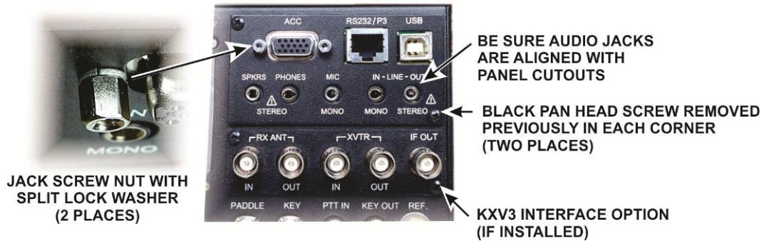
Figure 8. Mounting the new KIO3B Rear Panel Cover.
