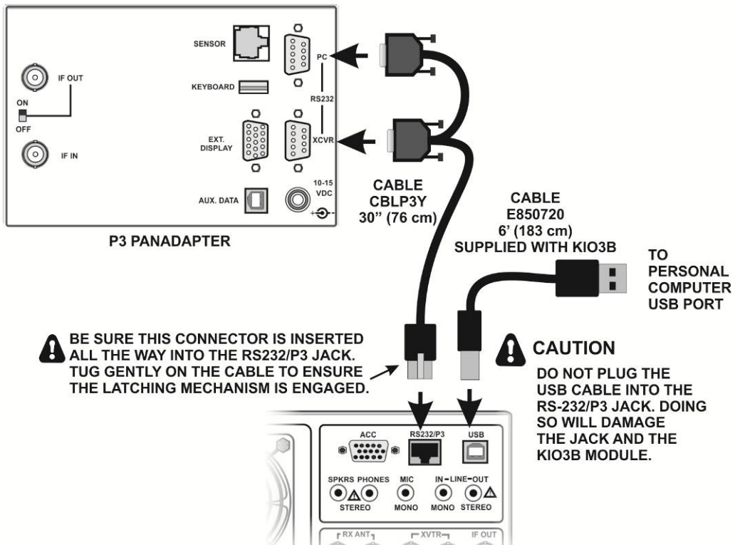
Figure 14. P3 Panadapter Cabling for USB Computer Interface.
