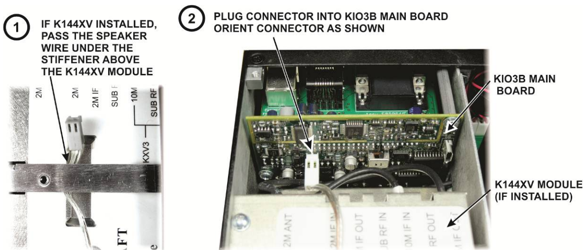
Figure 12. Connecting the Speaker Cable to the KIO3B Board.
