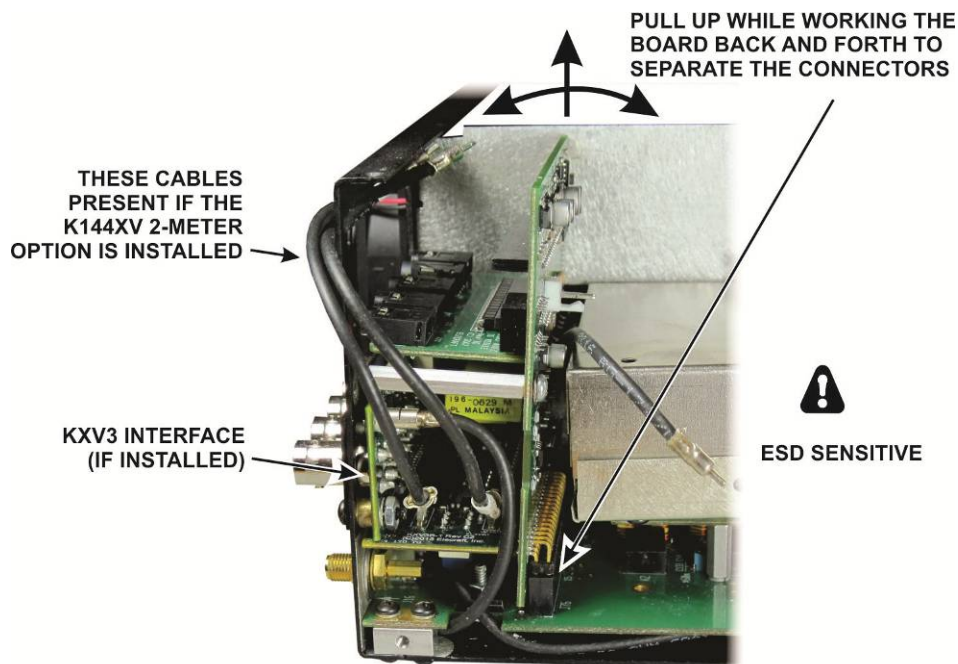
Figure 5. Removing the KIO3 Board.
